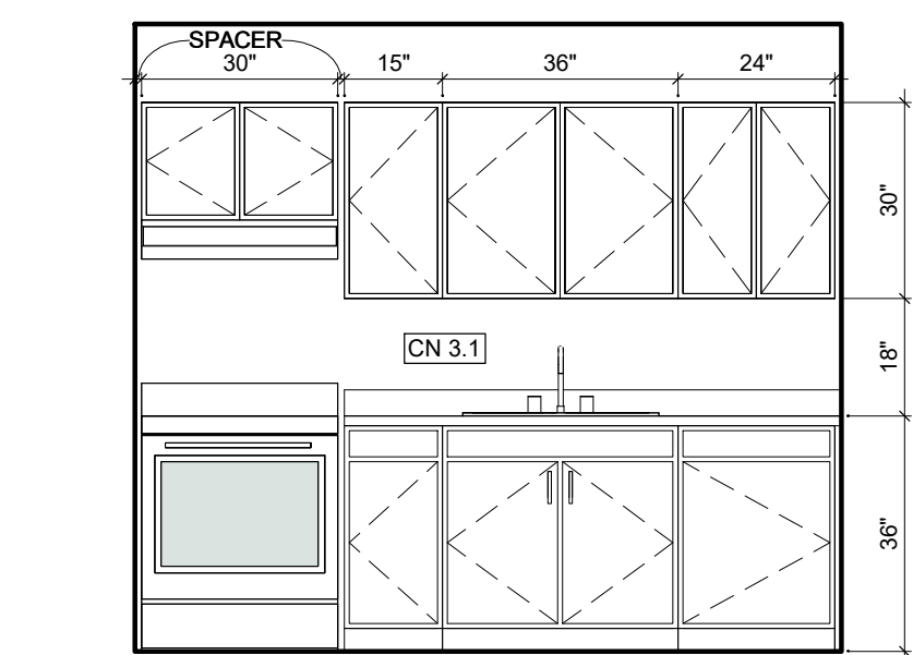
5 1, 2, & 3 BR TH - KIT. ELEV. A 3/8" = 1'-0"
