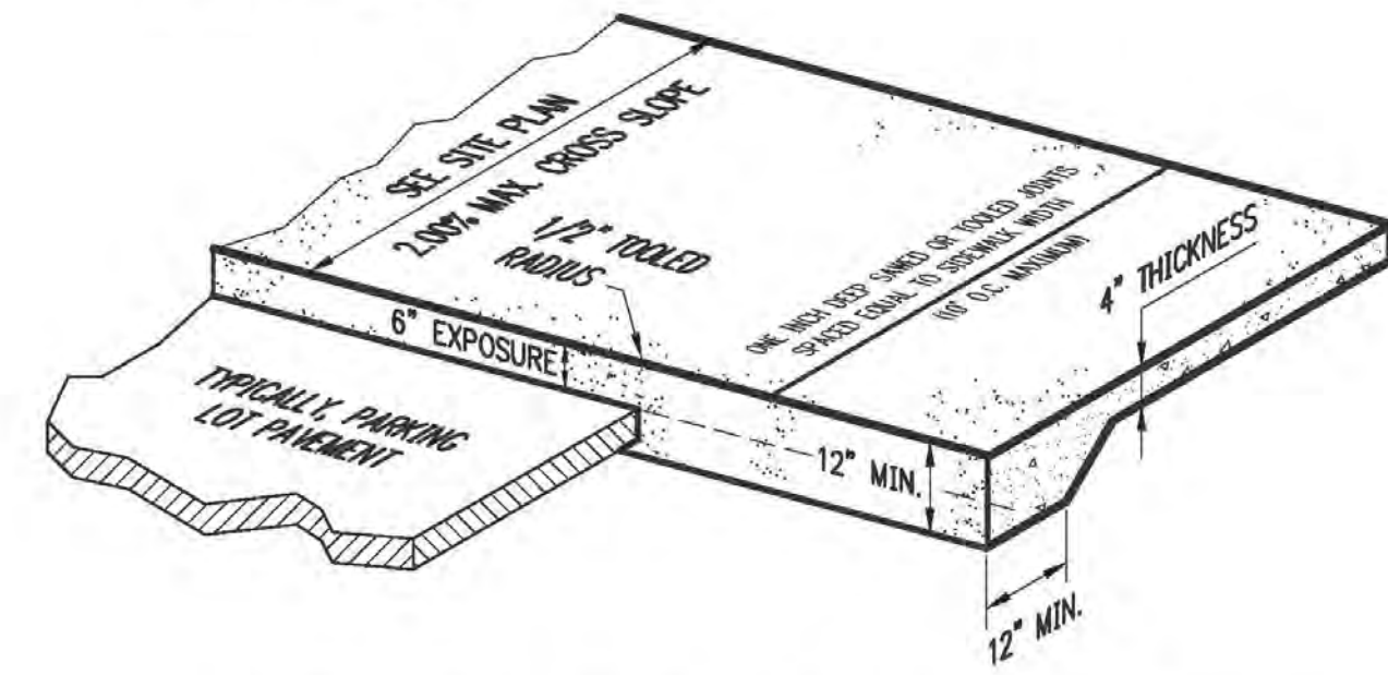
PRIVATE SIDEWALK WITH TURNED DOWN EDGE NTS
