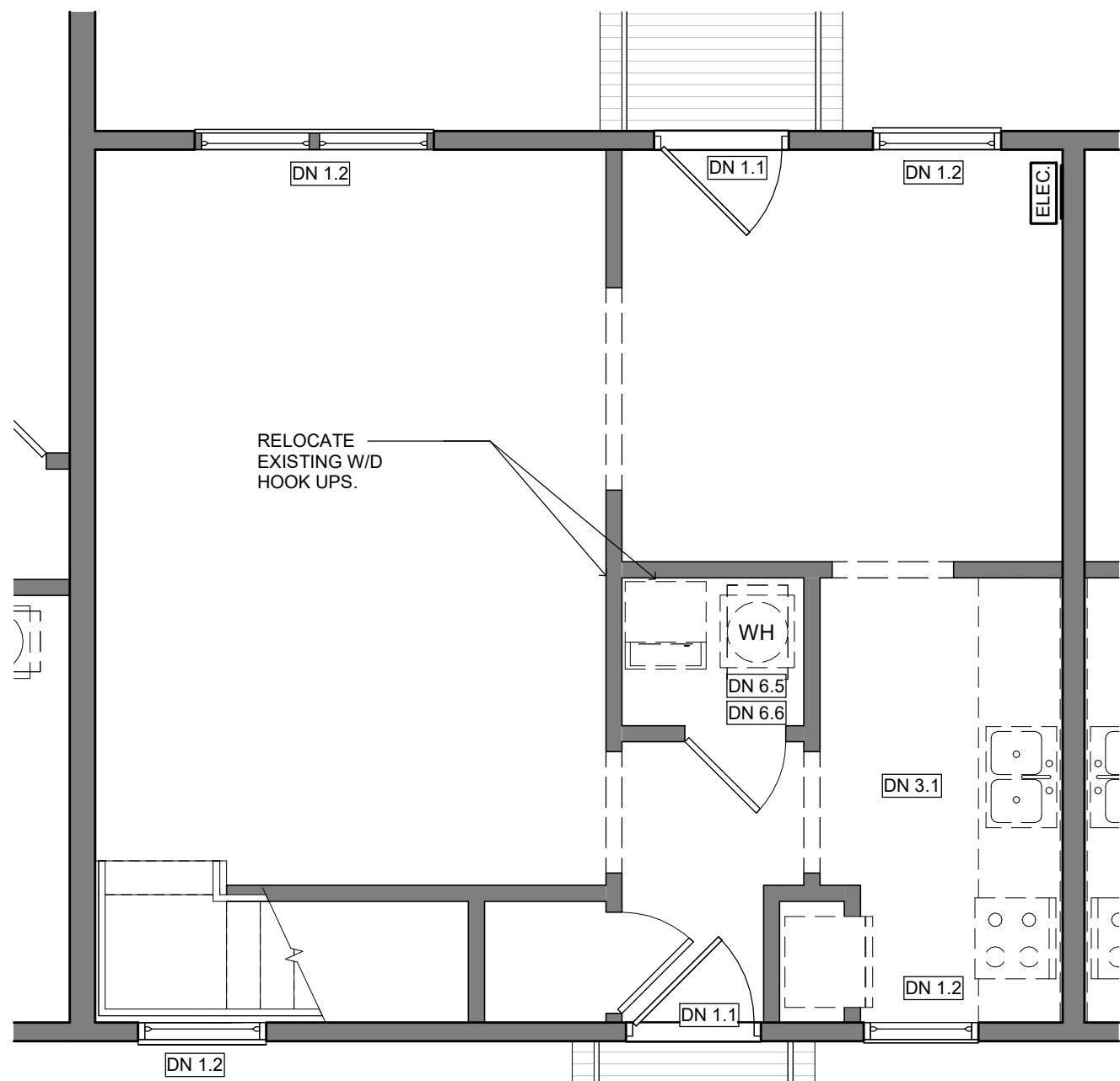
1 2BR TH ALT - FIRST FLOOR DEMO PLAN 1/4" = 1'-0"
