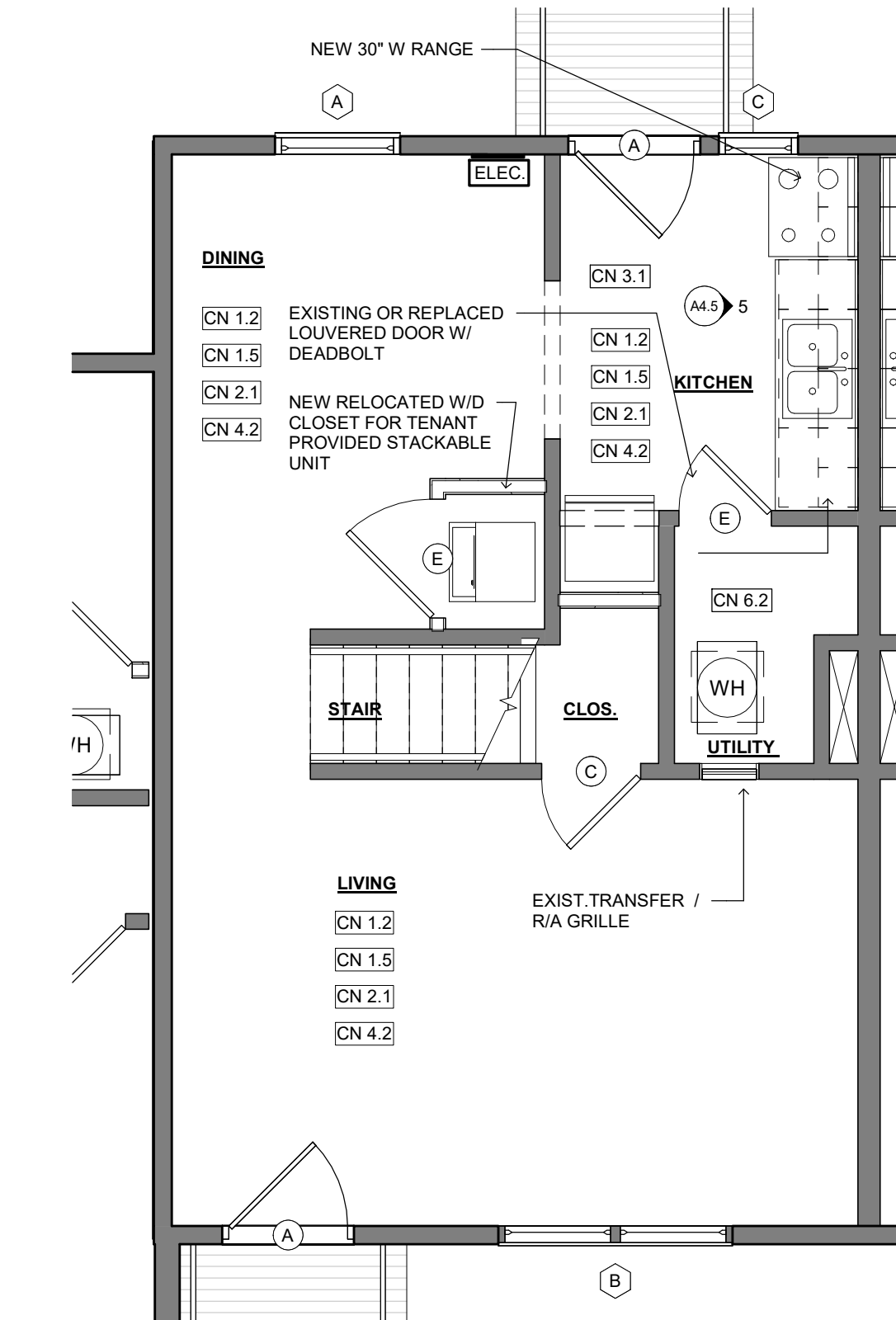
3 1BR TH - NEW FIRST FLOOR PLAN 1/4" = 1'-0"
