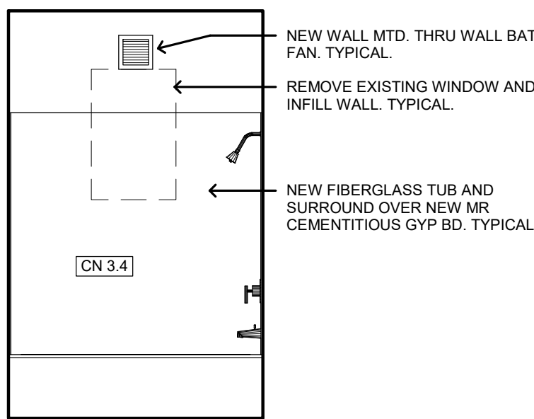
7 TYPICAL TUB ELEVATION ALL UNITS 3/8" = 1'-0"
