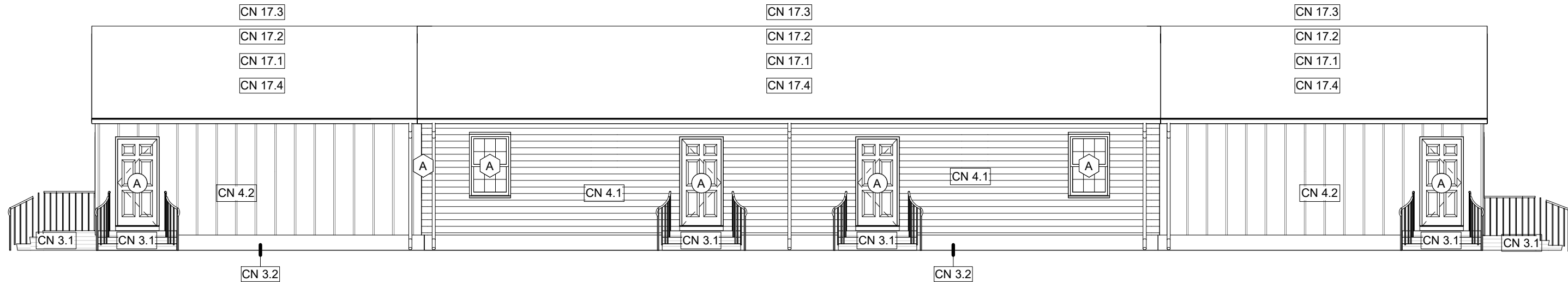
4 REAR ELEVATION - DEMO / NEW_BLDG TYPE VIII 1/8" = 1'-0"
