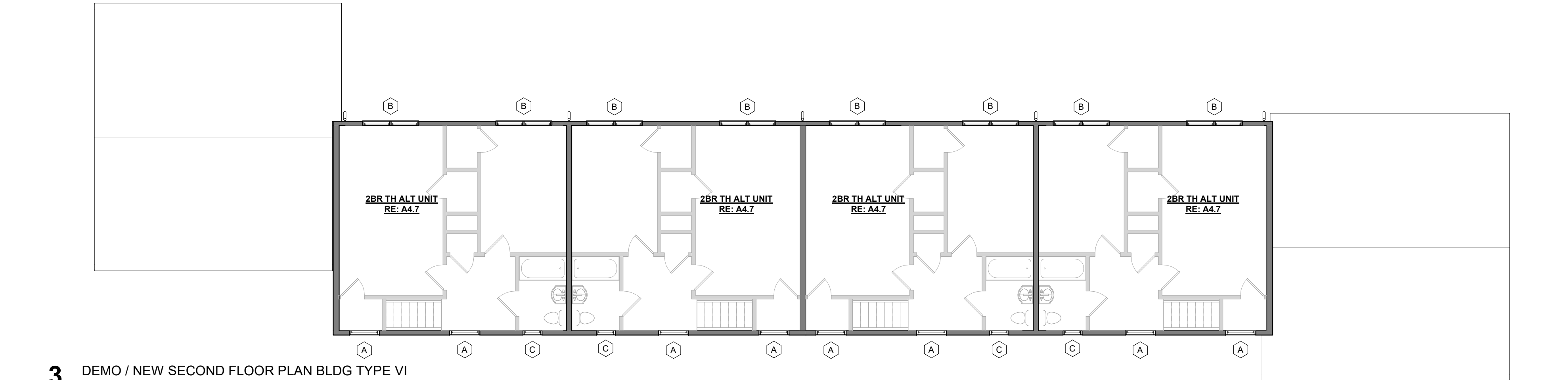
3 DEMO / NEW SECOND FLOOR PLAN BLDG TYPE VI 1/8" = 1'-0"
