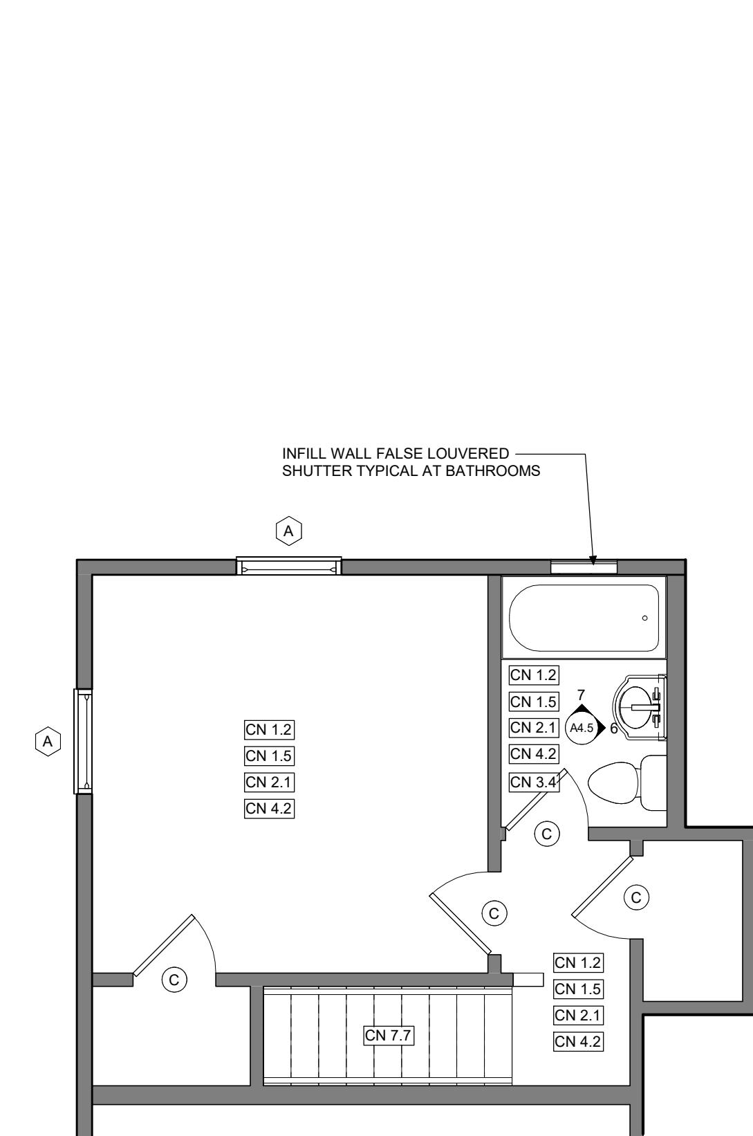
2 1BR TH - SECOND FLOOR DEMO PLAN 1/4" = 1'-0"
