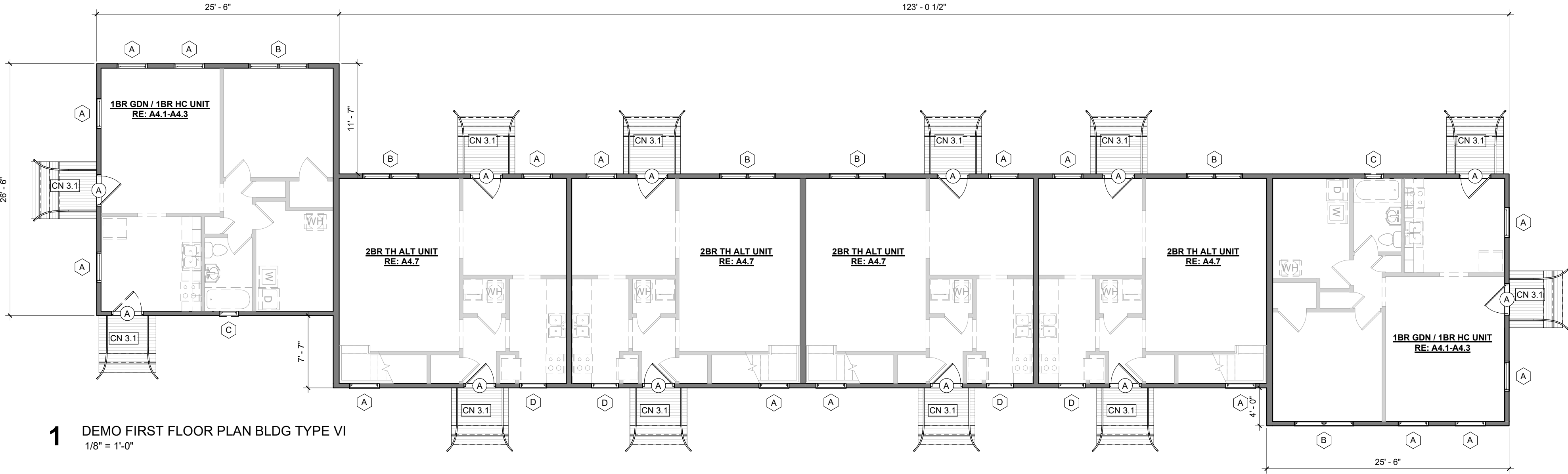
2 NEW FIRST FLOOR PLAN BLDG TYPE VI 1/8" = 1'-0"
