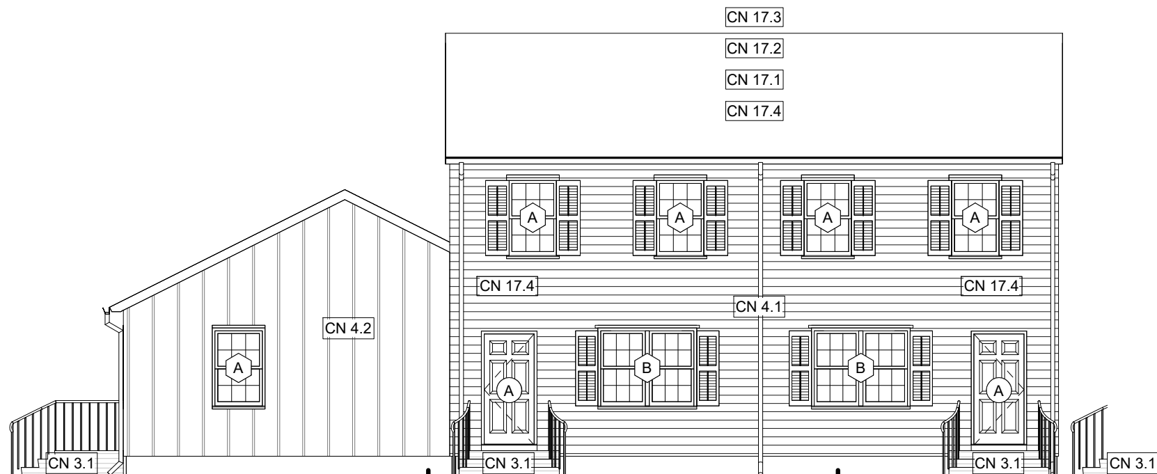
3 RIGHT ELEVATION - DEMO / NEW_BLDG TYPE XI 1/8" = 1'-0"
