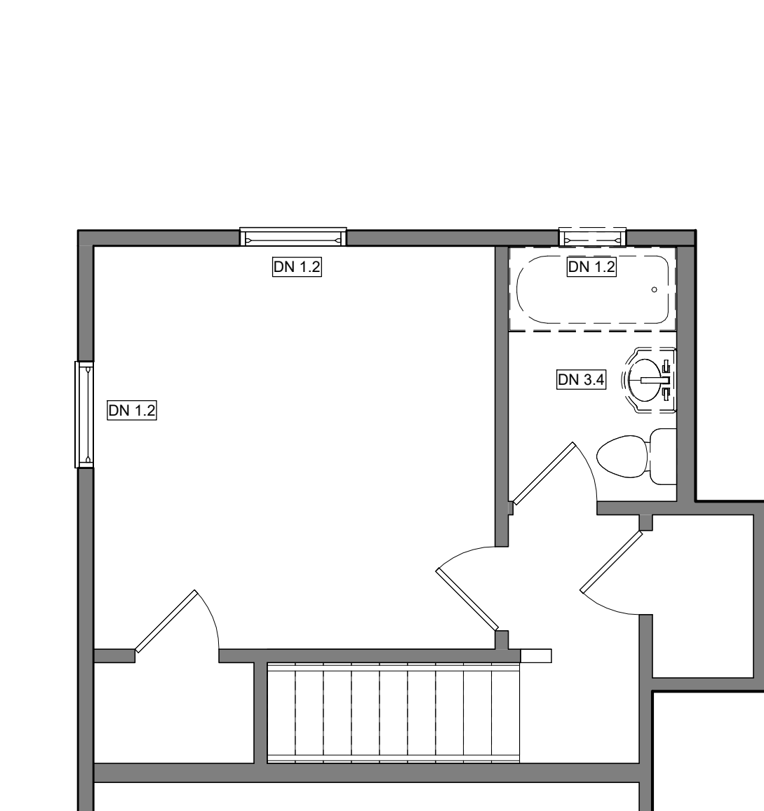
2 1BR TH - SECOND FLOOR DEMO PLAN 1/4" = 1'-0"
