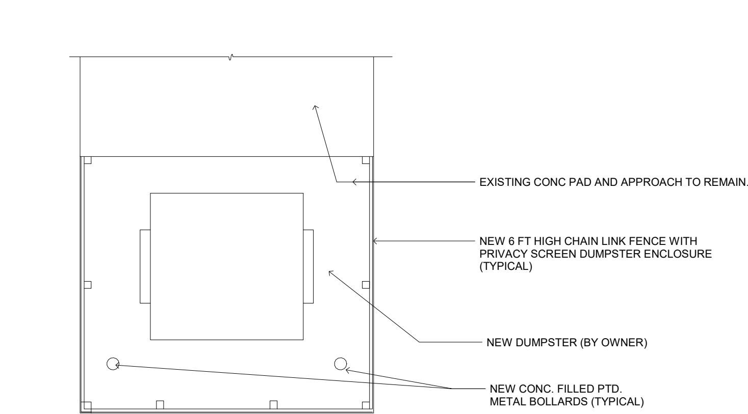
PLAN VIEW AT TYPICAL DUMPSTER ENCLOSURE 1 TYPICAL DUMPSTER ENCLOSURE DETAIL 1/4" = 1'-0"
