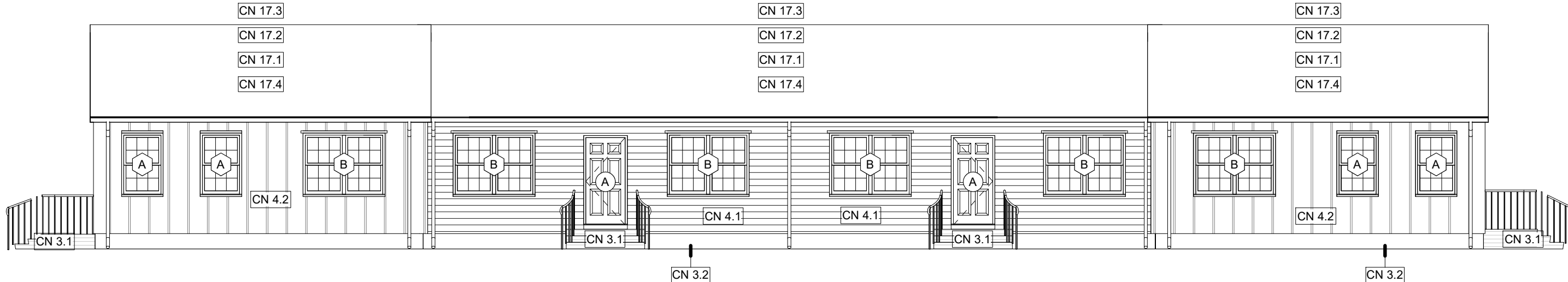
1 FRONT ELEVATION - DEMO / NEW_BLDG TYPE VIII 1/8" = 1'-0"
