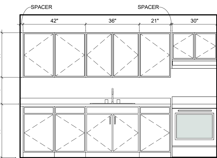
5 2BR TH ALT - KIT. ELEV. A 3/8" = 1'-0"
