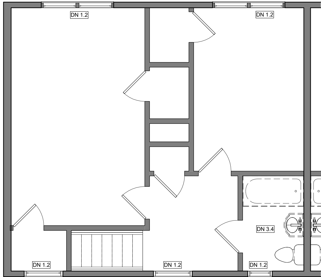
2 2BR TH ALT - SECOND FLOOR DEMO PLAN 1/4" = 1'-0"
