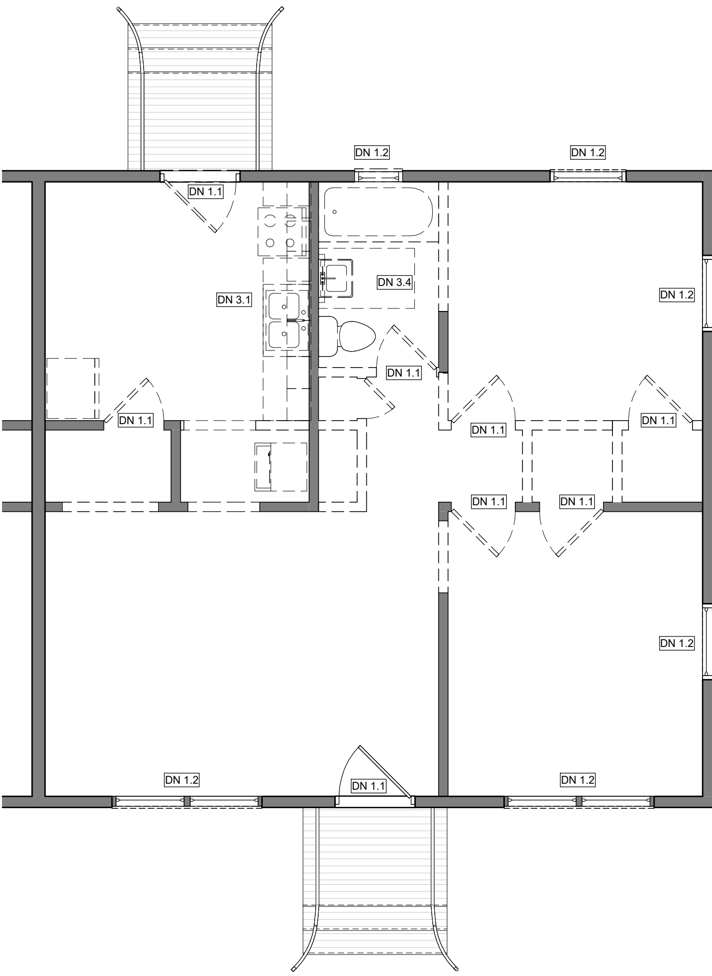
1 DEMO FLOOR PLAN 2BR HC - CONVERSION 1/4" = 1'-0"
