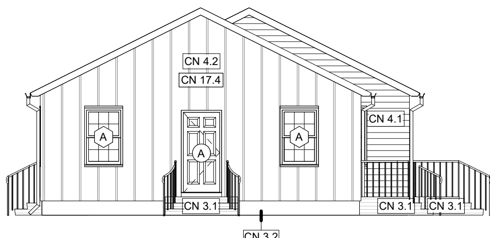
3 RIGHT ELEVATION - DEMO / NEW_BLDG TYPE VIII 1/8" = 1'-0"
