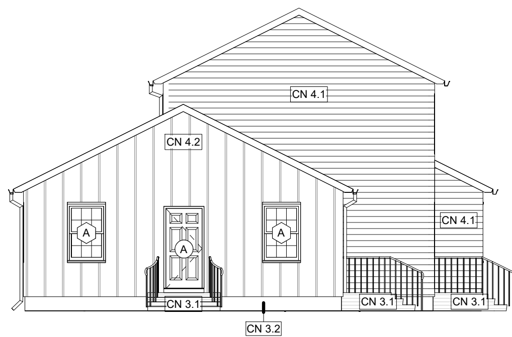
2 LEFT ELEVATION - DEMO / NEW_BLDG TYPE V 1/8" = 1'-0"
