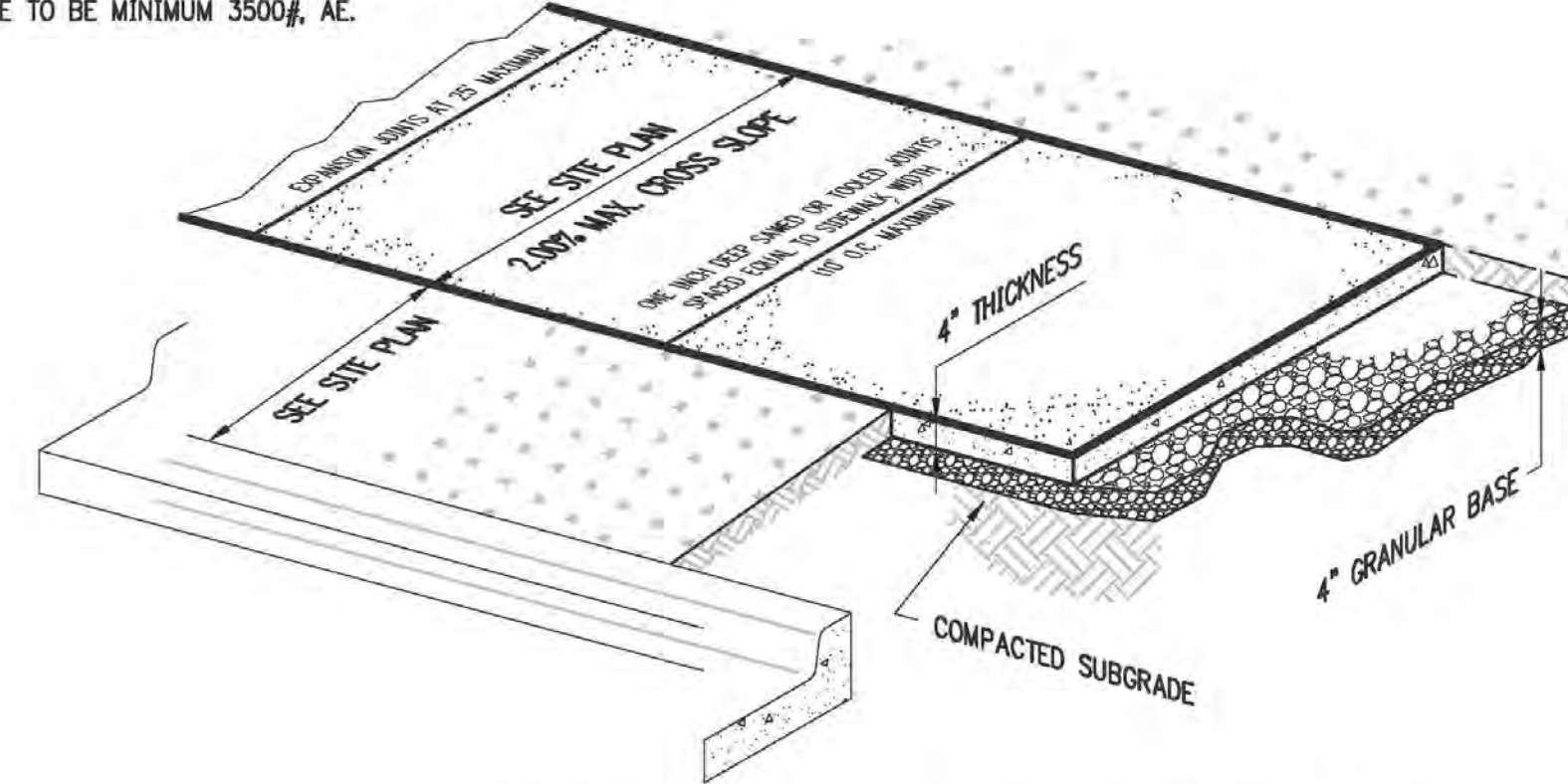
PRIVATE SIDEWALK WITH GREEN SPACE NTS
