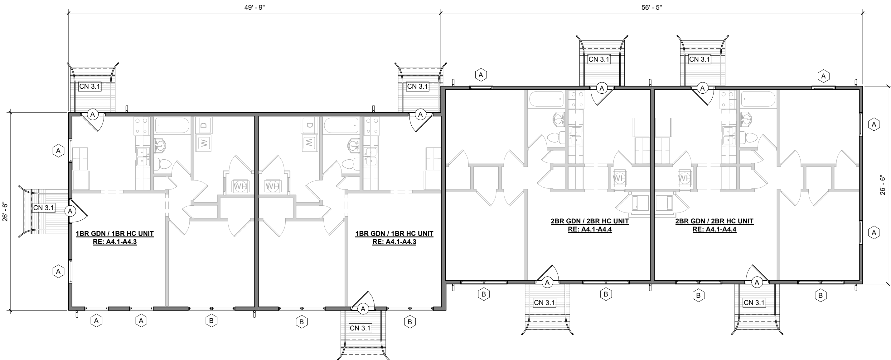
2 NEW FIRST FLOOR PLAN BLDG TYPE IV
