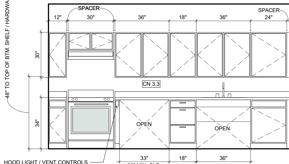
4 2BR GDN HC CONV - KIT. ELEV. B 3/8" = 1'-0"
