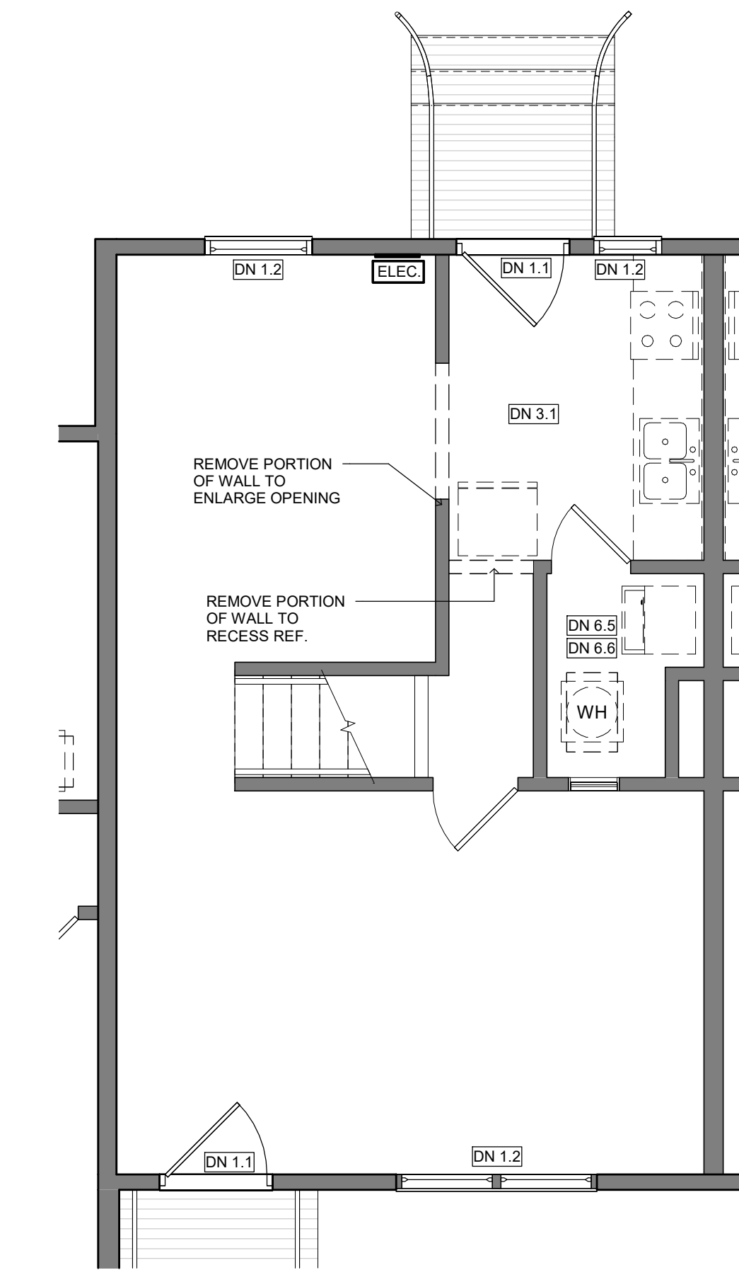
1 2BR TH - FIRST FLOOR DEMO PLAN 1/4" = 1'-0"
