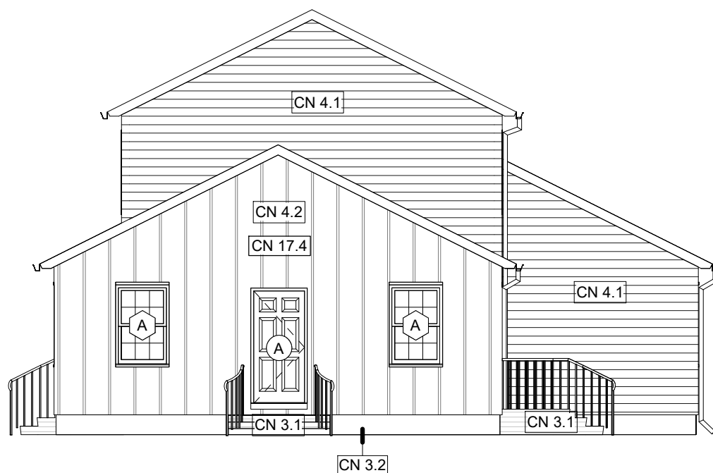
3 RIGHT ELEVATION - DEMO / NEW_BLDG TYPE VI 1/8" = 1'-0"
