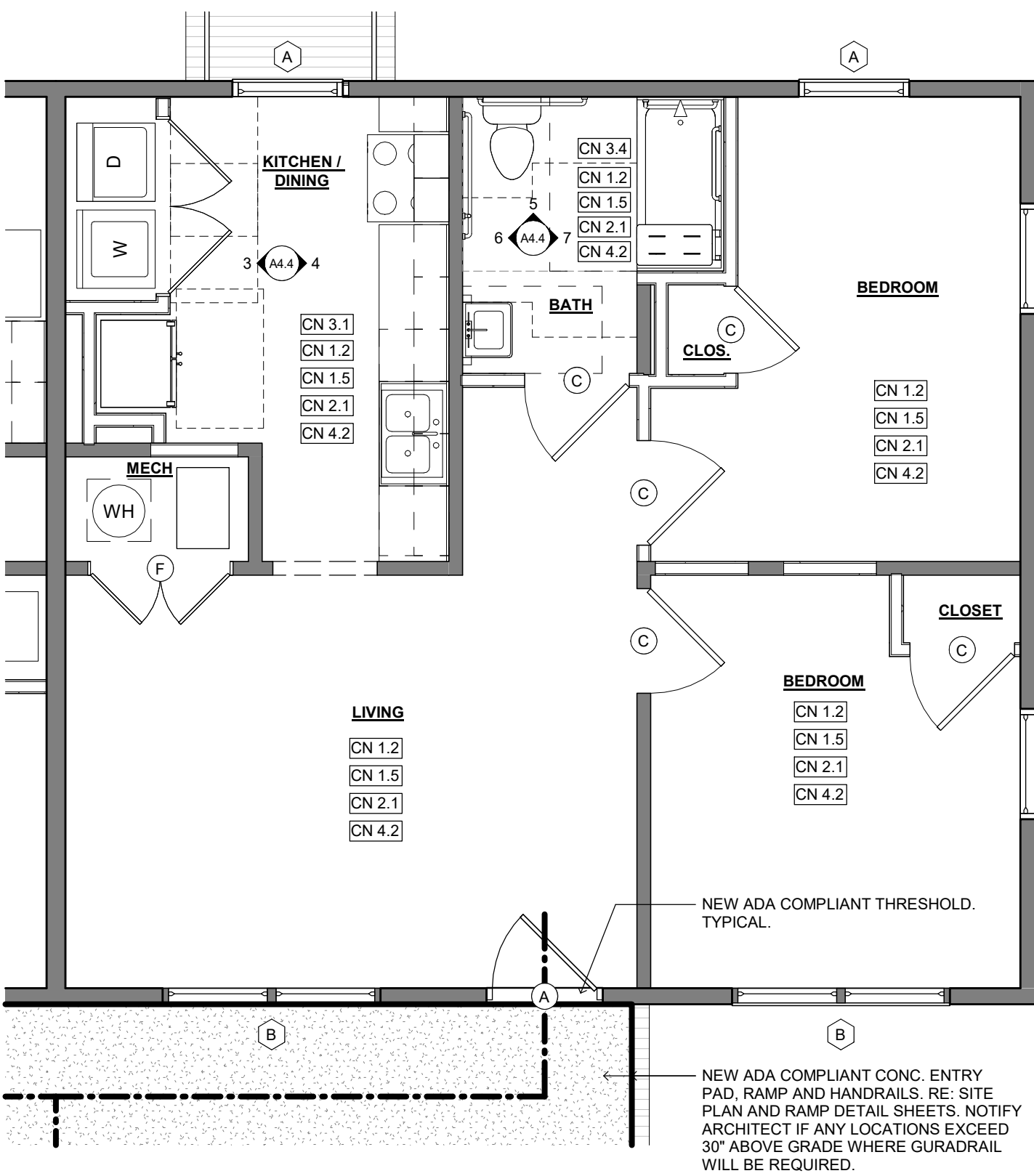
2 NEW FLOOR PLAN 2BR HC - CONVERSION 1/4" = 1'-0"
