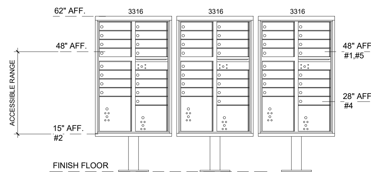
4 TYPICAL MAIL BOX CLUSTER ELEVATION (MK) 1/2" = 1'-0"
