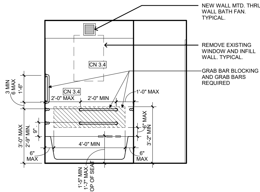
7 2BR GDN HC CONV - BATH ELEV. C 3/8" = 1'-0"
