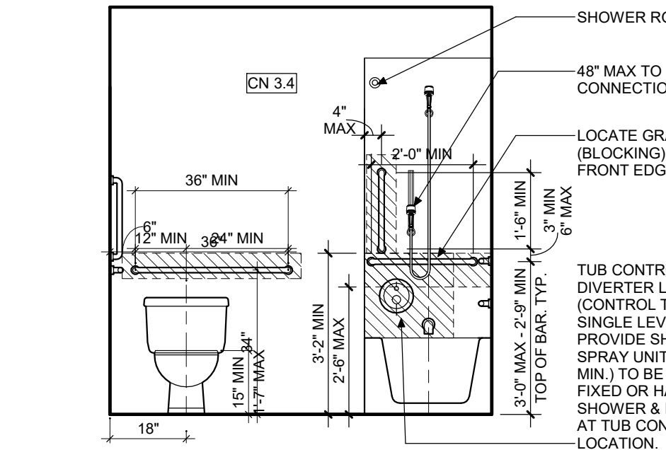
5 2BR GDN HC CONV - BATH ELEV. A 3/8" = 1'-0"
