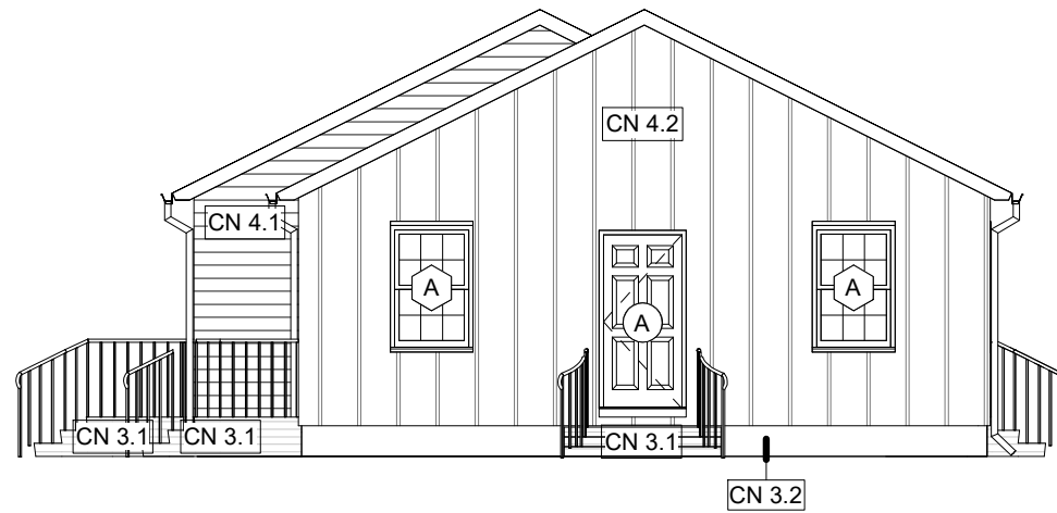
2 LEFT ELEVATION - DEMO / NEW_BLDG TYPE VIII 1/8" = 1'-0"
