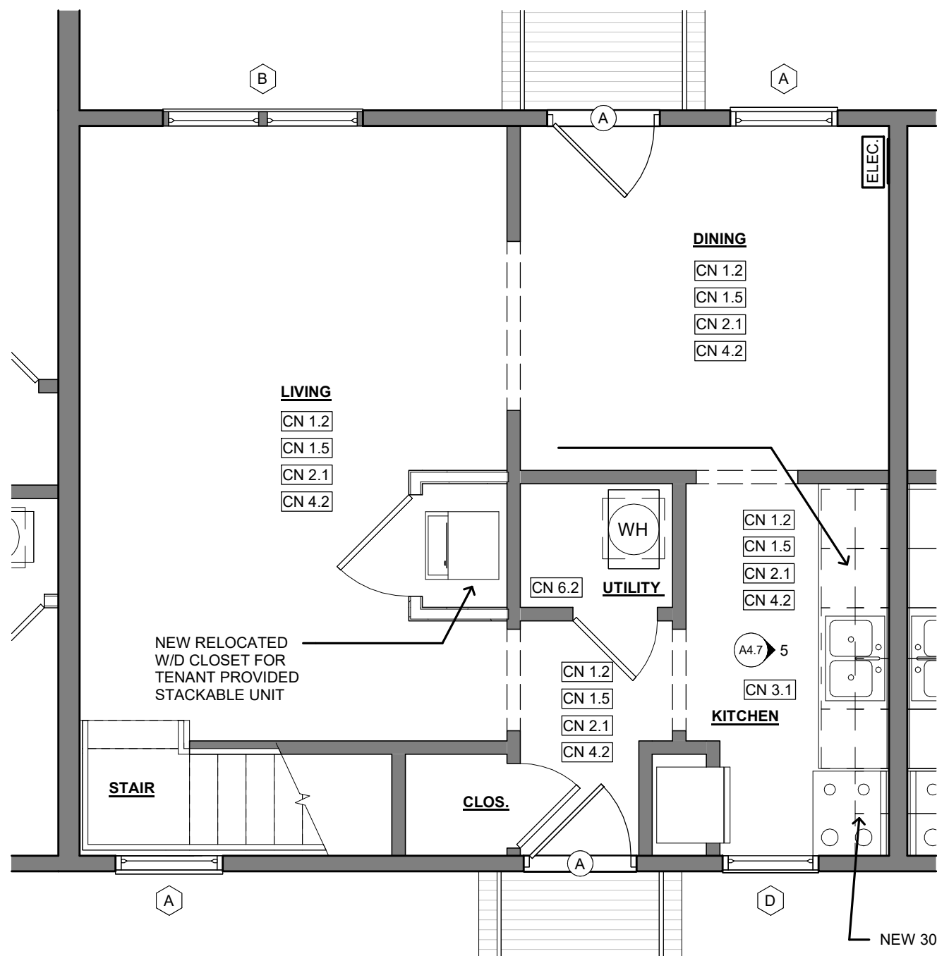
3 2BR TH ALT - NEW FIRST FLOOR PLAN 1/4" = 1'-0"
