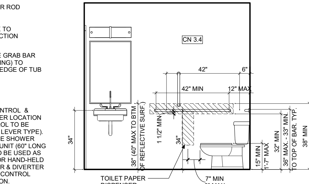
6 2BR GDN HC CONV - BATH ELEV. B 3/8" = 1'-0"
