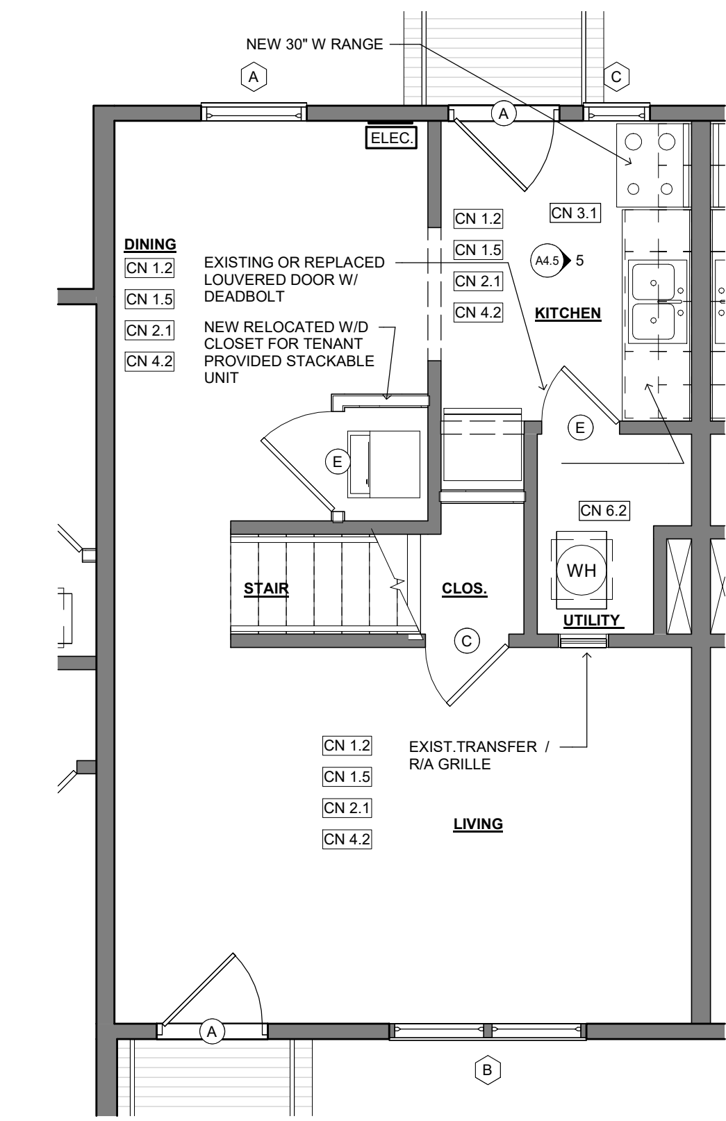
3 2BR TH - NEW FIRST FLOOR PLAN 1/4" = 1'-0"
