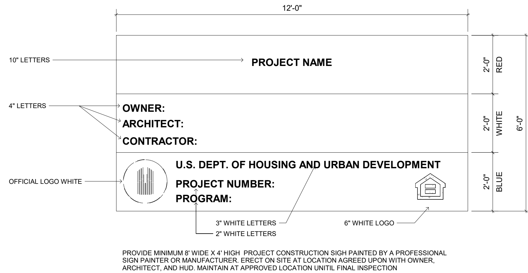
2 CONSTRUCTION JOB SITE SIGN 3/4" = 1'-0"
